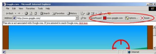
Figure 1: SpoofGuard
