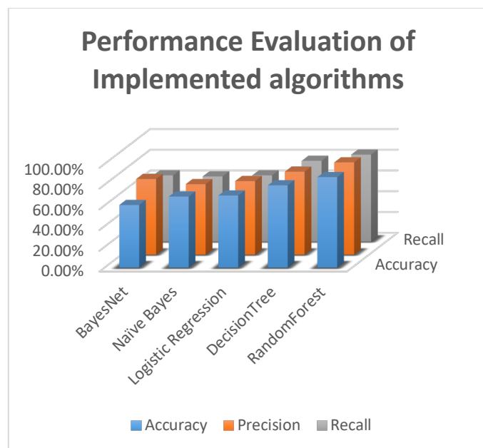
Figure 7: Performance evaluation of implemented algorithm
