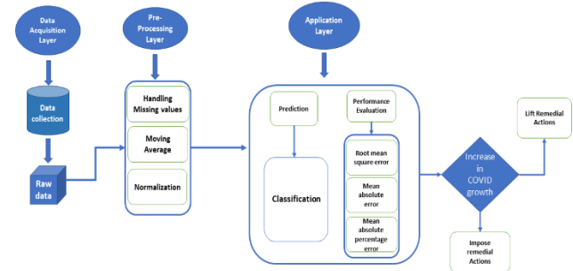
Figure 4: Proposed System Architecture
